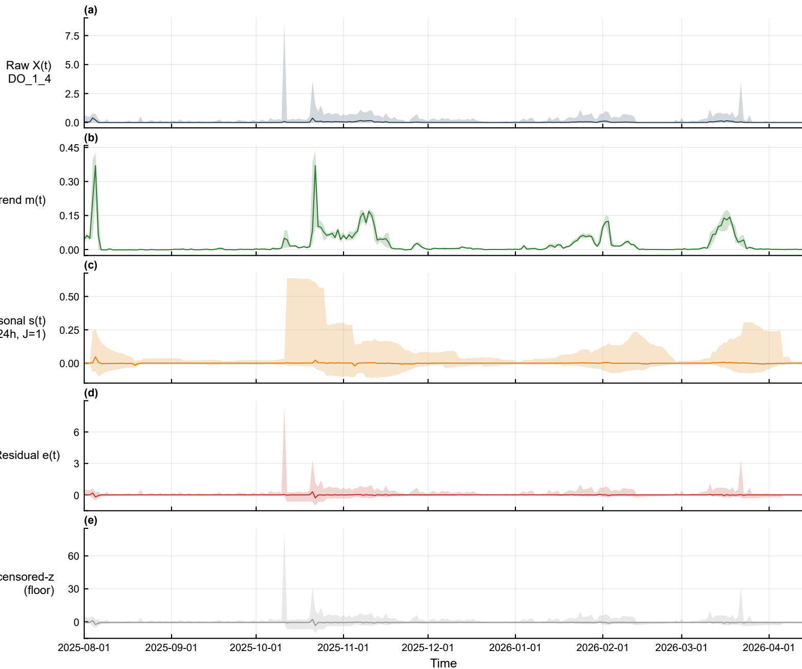
Full-span daily overview — DO_1_4 (post_anoxic, min) [2025-08-01~2026-04-13]
